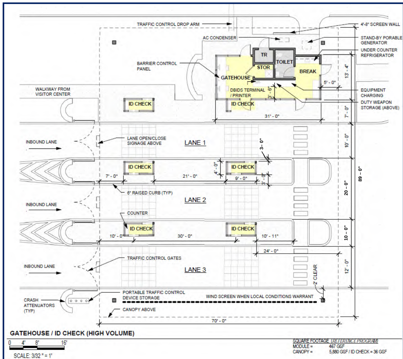
Figure 5-11 Model ID Check Island Details – High Volume
