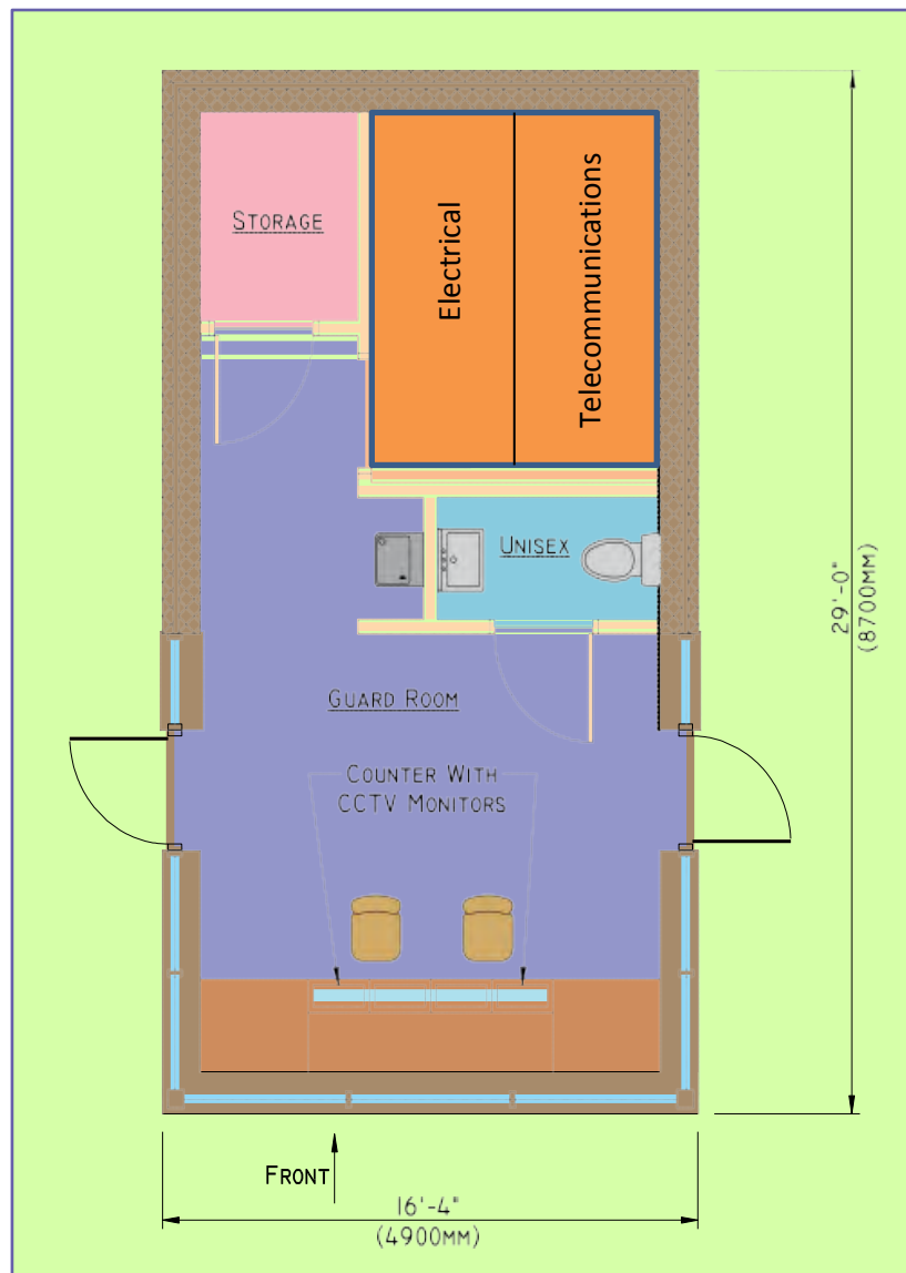
Figure 5-10 Model Gatehouse Floor Plan
