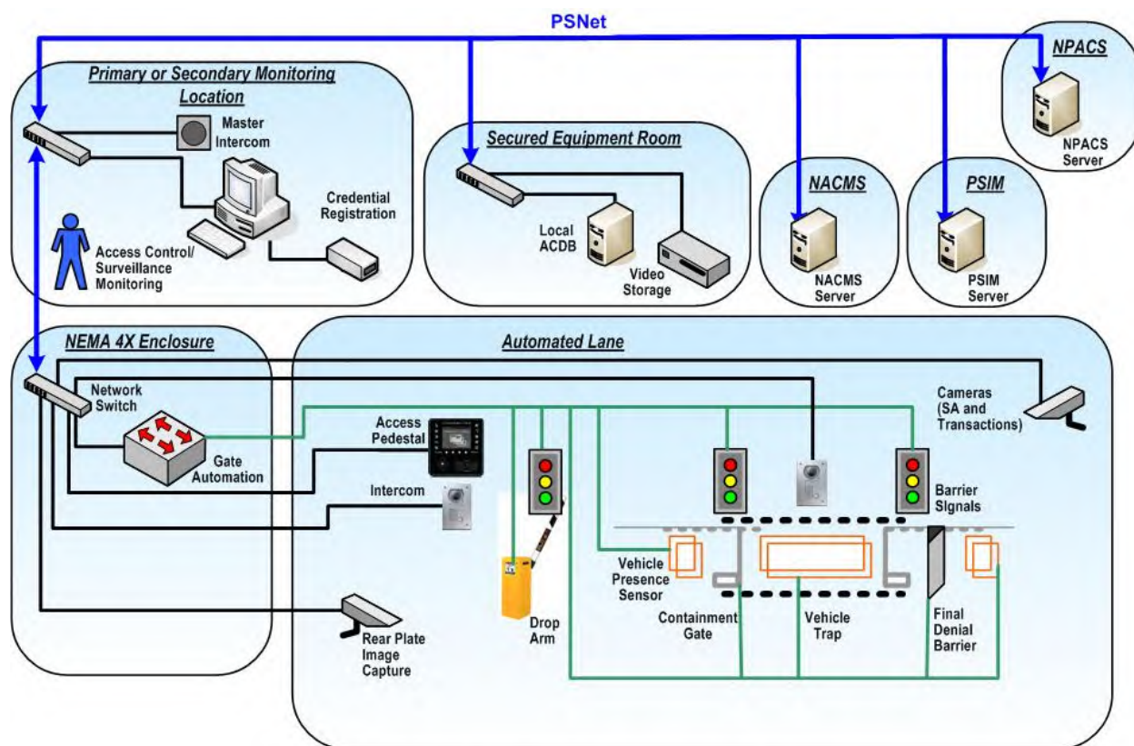
Automated Vehicle Gate – Low Volume
