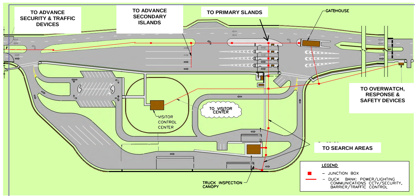
Figure 5-14 Model Duct Bank Plan
